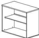
OPEN SHELF CABINET iAO 880 800W x 400D x 820H
