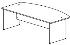
EXECUTIVE TABLE iEXT 180A 1800W x 900D x 750H
