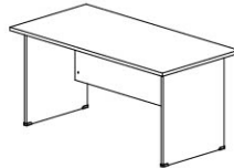
STANDARD TABLE iEXT 126 1200W x 600D x 750H
