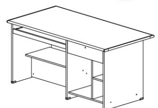
COMPUTER WORKSTATION iSC 3000 1210W x 620D x 750H
