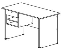
WRITING TABLE iEW 1836 900W x 450D x 738H
